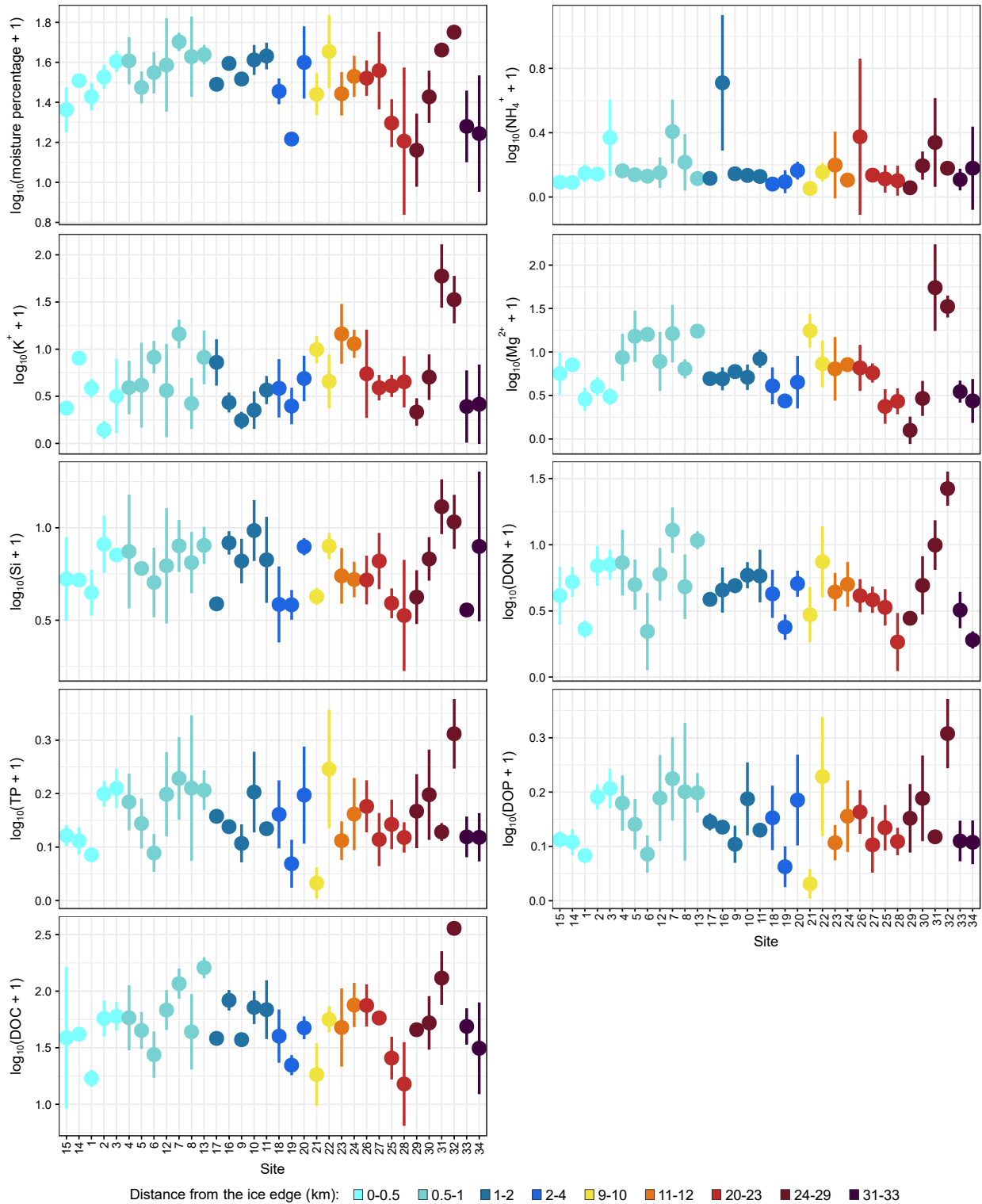
Figure D1 continued. Geochemical trends across the proglacial sampling sites. Values are shown as mean \pm standard deviation for each site. These figures report the variables that were not significantly correlated ( p -value \geq 0.05 ) to site distance from the ice edge in the Spearman's rank correlation tests (results shown in Table 1).
