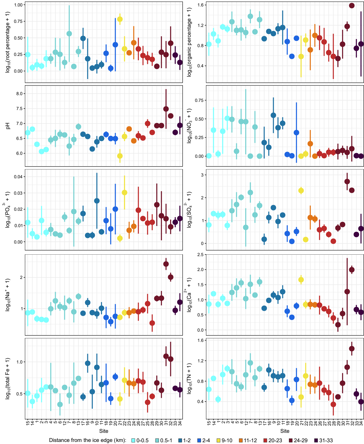
Figure D1. Geochemical trends across the proglacial sampling sites. Values are shown as mean \pm standard deviation for each site. These figures report the variables that were significantly correlated ( p -value < 0.05 ) to site distance from the ice edge in the Spearman's rank correlation tests (results shown in Table 1).
