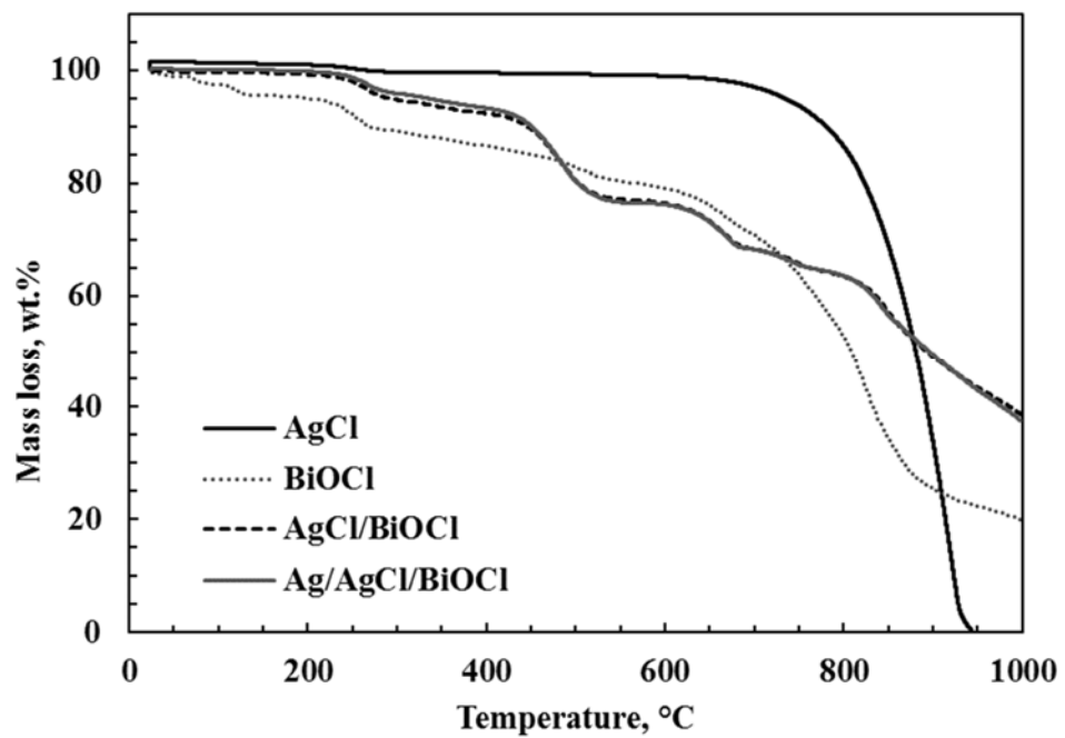
Figure 2: TGA curves of as-synthesized particles
