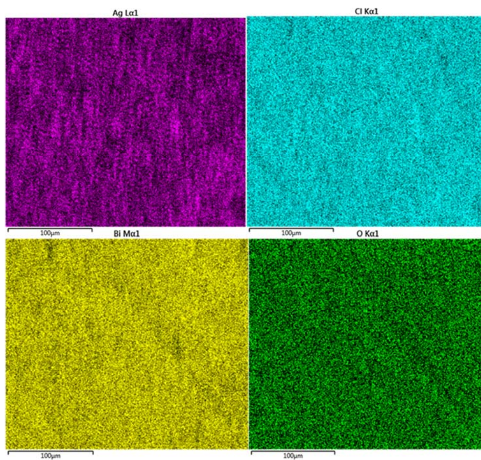
Figure 1: EDS mapping of Ag/AgCl/BiOCl
