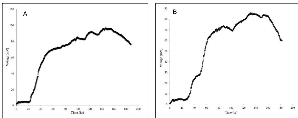
Figure 2: Voltage generation over the operation cycle time with each MFC having an initial glucose substrate concentration of 5.56 mM
