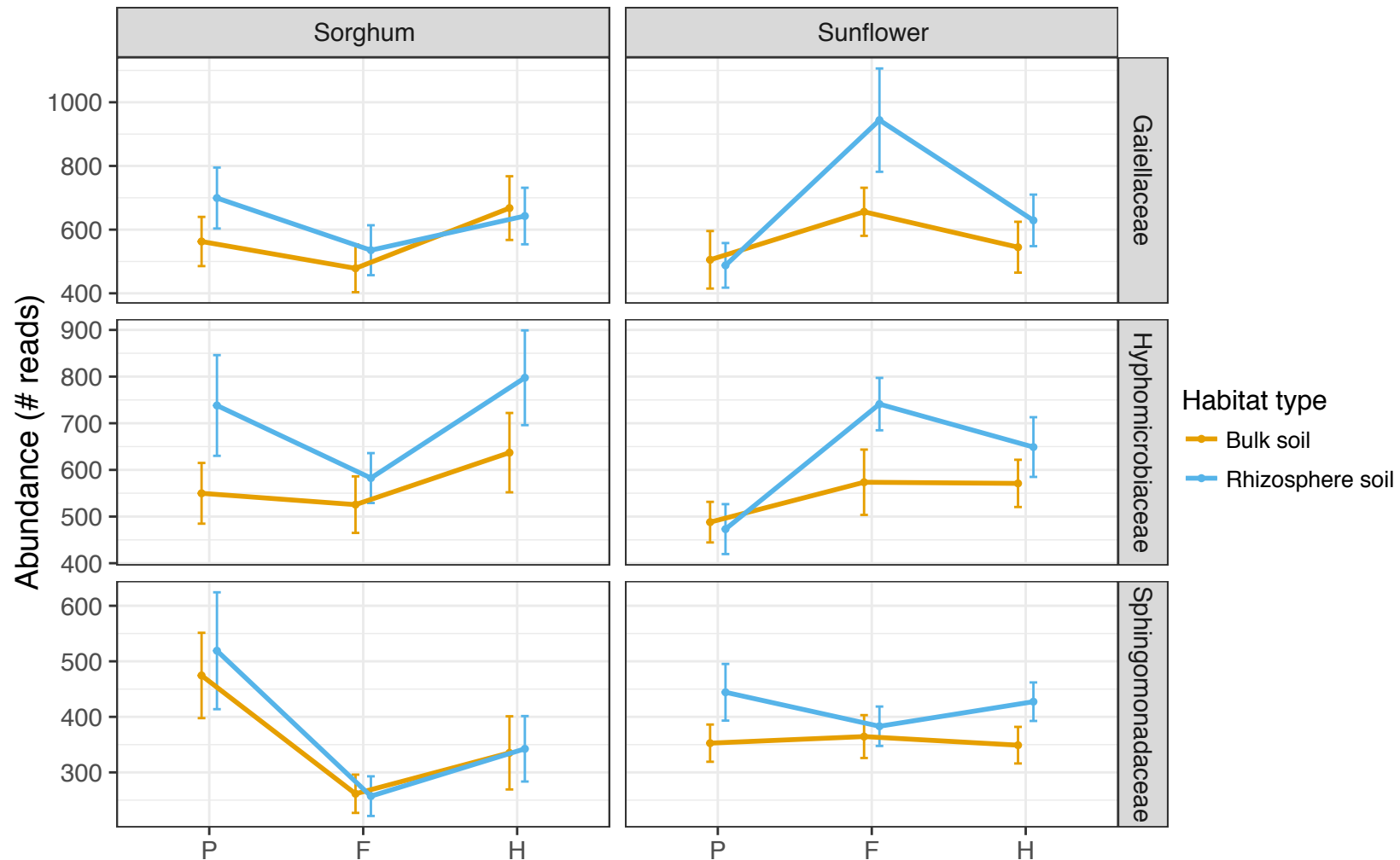
Supplementary data Fig. S12. Abundance of the families enriched in each habitat type (bulk and rhizosphere soils).
