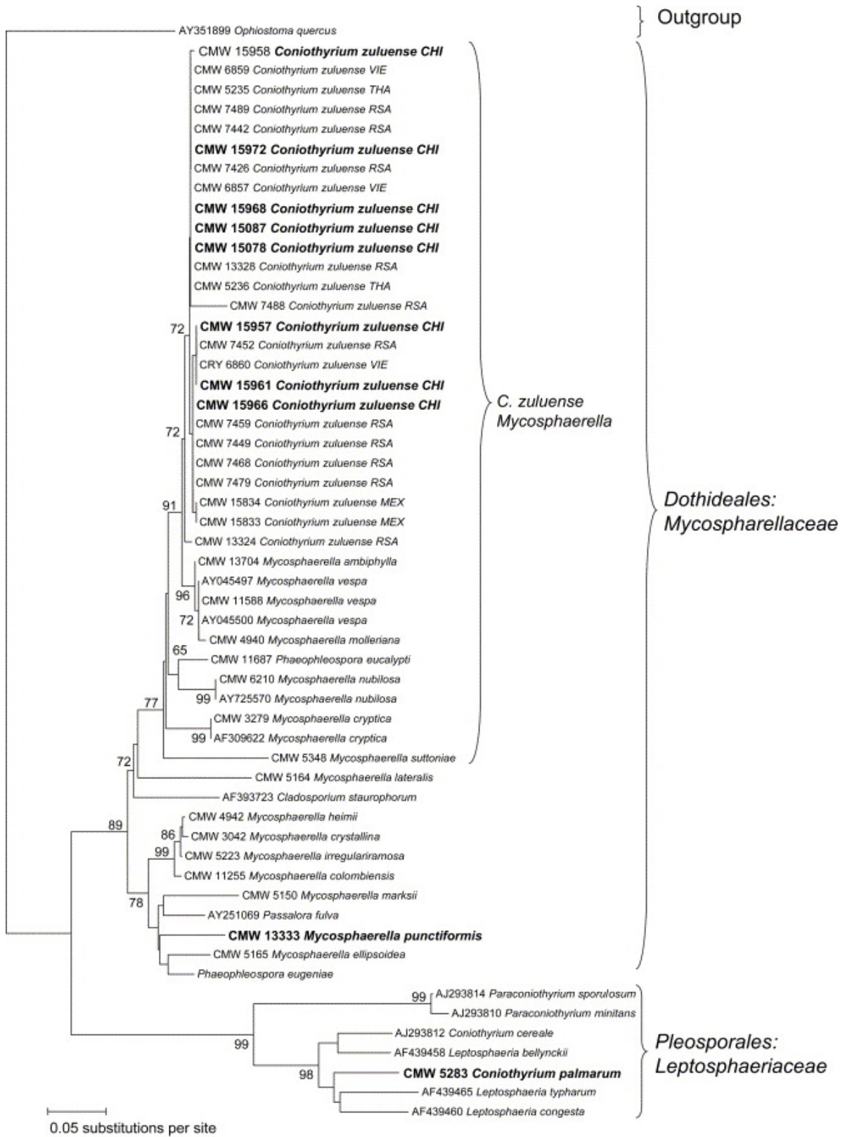
Fig 2. Phylogram obtained from ITS sequencing data gene using the Kimura with two parameters nucleotide substitution model and neighbour-joining. Bootstrap support
