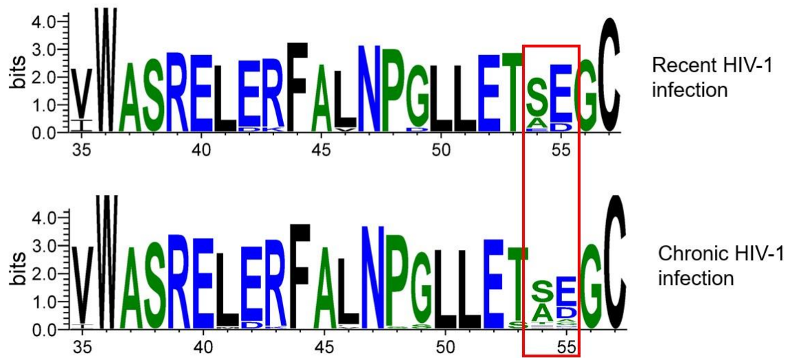
Supplementary figure 3: Diversity at amino acid positions 54 and 55. In study sequences, amino acid sites S54 and E55 showed more diversity in chronic sequences when compared to recent sequences. HIV-1 – Human Immunodeficiency virus type 1.
