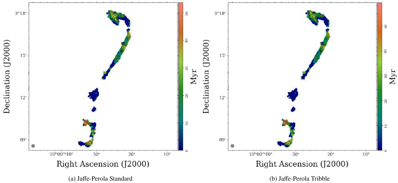
Figure 8. As Fig. 6, but for GRG3. The magnetic field is 0.587 \mu\text{G} , and the resulting maximum ages are 64 \pm 31 and 67 \pm 36 Myr according to the JP and JP Tribble models, respectively. Percentage uncertainty contours are shown in black at 40 per cent, 60 per cent, and 80 per cent.
