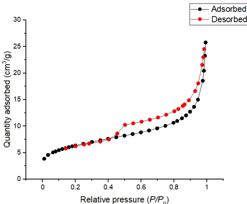
Figure S1. The nitrogen a nitrogen adsorption–desorption isotherms of the non-KOH activated 3D black TiO 2 , Ag, N@rGO solar absorber.
