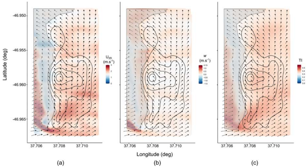
Fig. S10. Two-dimensional wind map, extracted at a constant 1 m.a.g.l. from numerical simulation of a south-westerly wind ( \theta = 225^\circ ) freestream condition over Marion Island. Crash site density contours (black, solid lines) are displayed with the outline of the base of the Ridge (semi-transparent grey area). Each grid point is denoted by an arrow indicating the wind direction (local wind direction) with backgrounds coloured by two-dimensional horizontal velocity magnitude ( U_{2D} ; a), the vertical wind component ( w ; b) and the isotropic turbulence intensity (TI; c)
