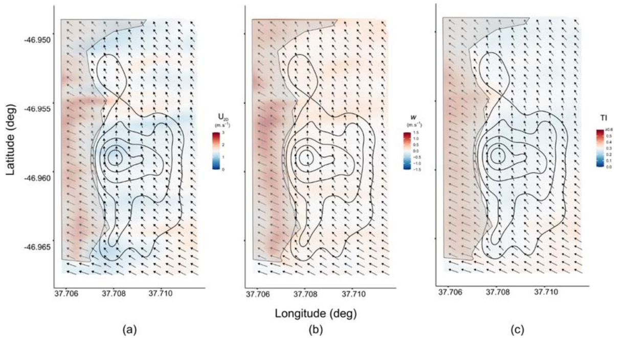
Fig. S8. Two-dimensional wind map, extracted at a constant 1 m.a.g.l. from numerical simulation of a south-easterly wind ( \theta = 135^\circ ) freestream condition over Marion Island. Crash site density contours (black, solid lines) are displayed with the outline of the base of the Ridge (semi-transparent grey area). Each grid point is denoted by an arrow indicating the wind direction (local wind direction) with backgrounds coloured by two-dimensional horizontal velocity magnitude ( U_{2D} ; a), the vertical wind component ( w ; b) and the isotropic turbulence intensity (TI; c)
