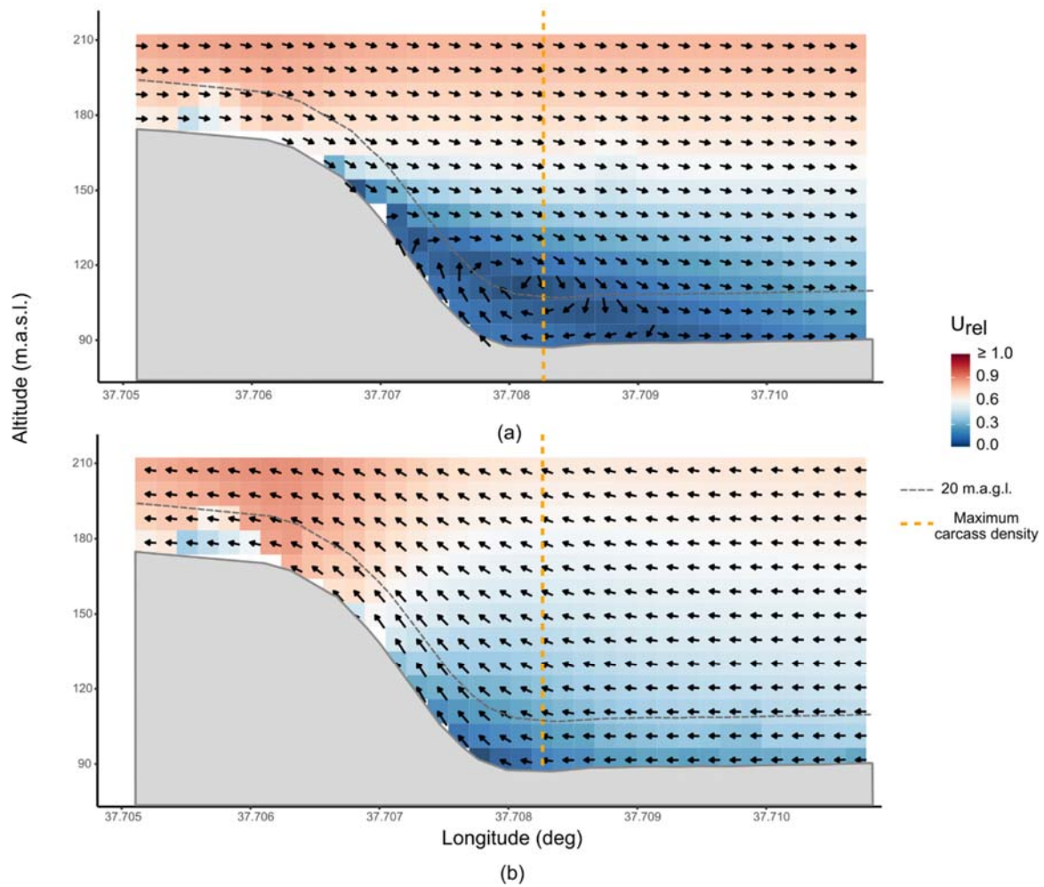
Fig. S3. Cross-section at a constant latitudinal line ( -46.957^\circ ) corresponding to the maximum carcass density. Black arrows indicate two-dimensional vectors with the vertical and longitudinal velocity components with the background tiles coloured by the relative velocity ( U_{rel} ; velocity magnitude divided by U_{ref} = 3 \text{ m.s}^{-1} ), for westerly (a) and easterly (b) winds. The grey area is an approximation of the Ridge slope at this latitude, the grey dashed line is a constant 20 m.a.g.l line above the Valley and Ridge and the orange dashed line indicates the longitudinal line crossing the maximum carcass density.
