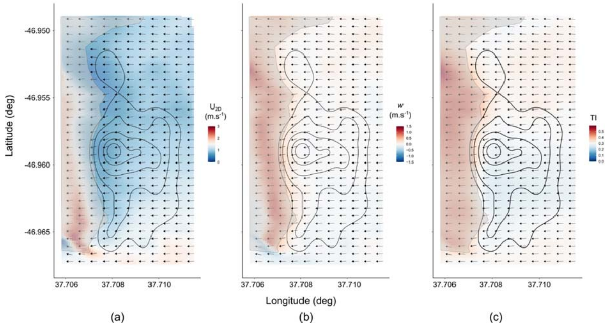
Fig. S7. Two-dimensional wind map, extracted at a constant 1 m.a.g.l. from numerical simulation of an easterly wind ( \theta = 90^\circ ) freestream condition over Marion Island. Crash site density contours (black, solid lines) are displayed with the outline of the base of the Ridge (semi-transparent grey area). Each grid point is denoted by an arrow indicating the wind direction (local wind direction) with backgrounds coloured by two-dimensional horizontal velocity magnitude ( U_{2D} ; a), the vertical wind component ( w ; b) and the isotropic turbulence intensity (TI; c).
