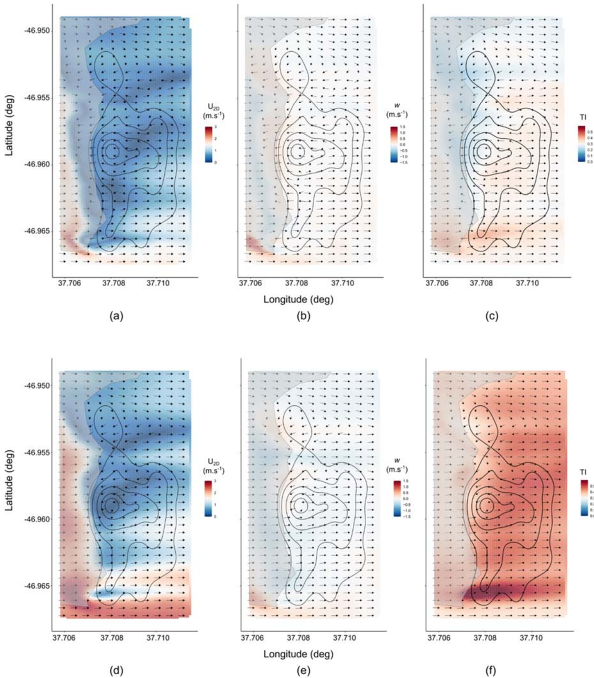
Fig. S11. Two-dimensional wind map, extracted at a constant 1 m.a.g.l. (a-c) and 20 m.a.g.l. (d-f) from numerical simulation of a westerly wind ( \theta = 270^\circ ) freestream condition over Marion Island. Crash site density contours (black, solid lines) are displayed with the outline of the base of the Ridge (semi-transparent grey area).
