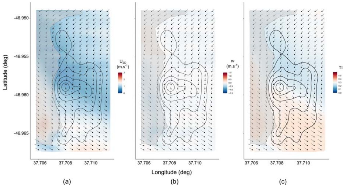
Fig. S12. Two-dimensional wind map, extracted at a constant 1 m.a.g.l. from numerical simulation of a north-westerly wind ( \theta = 315^\circ ) freestream condition over Marion Island. Crash site density contours (black, solid lines) are displayed with the outline of the base of the Ridge (semi-transparent grey area). Each grid point is denoted by an arrow indicating the wind direction (local wind direction) with backgrounds coloured by two-dimensional horizontal velocity magnitude ( U_{2D} ; a), the vertical wind component ( w ; b) and the isotropic turbulence intensity (TI; c).
