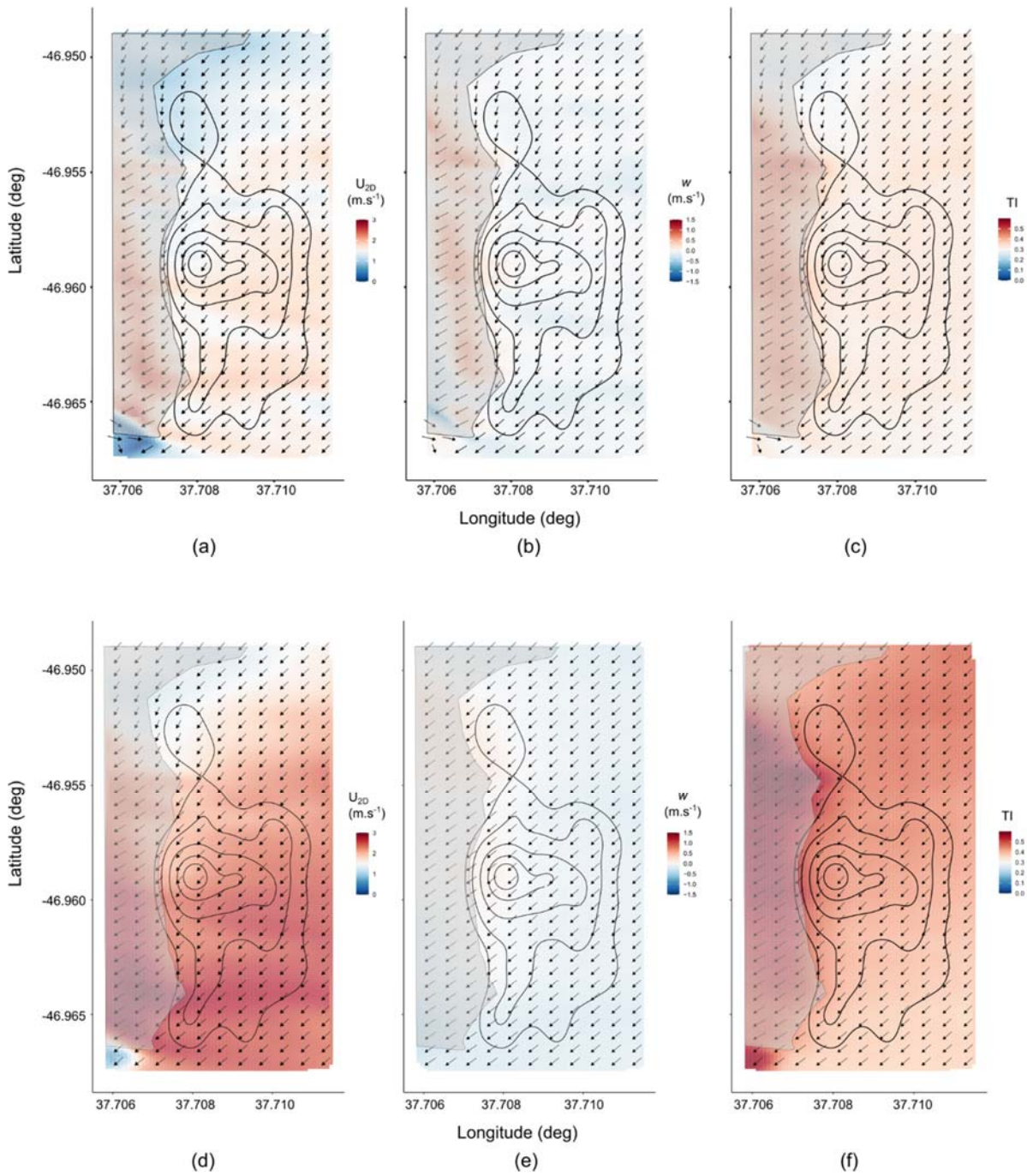
Fig. S6. Two-dimensional wind map, extracted at a constant 1 m.a.g.l. (a-c) and 20 m.a.g.l. (d-f) from numerical simulation of a north-easterly wind ( \theta = 45^\circ ) freestream condition over Marion Island. Crash site density contours (black, solid lines) are displayed with the outline of the base of the Ridge (semi-transparent grey area).
