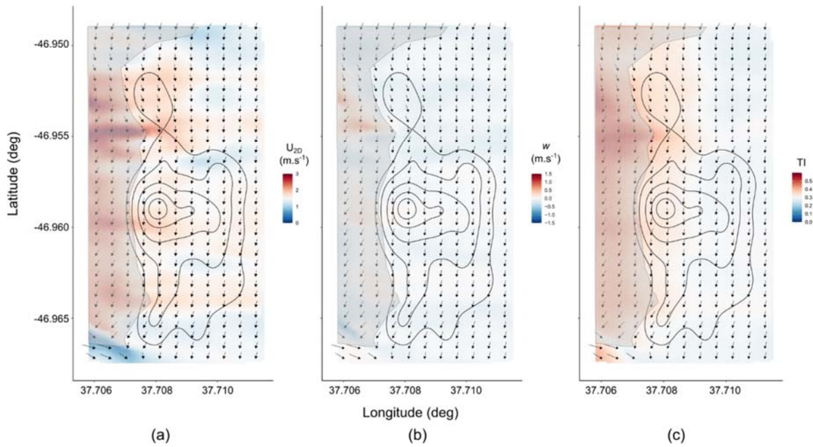
Fig. S5. Two-dimensional wind map, extracted at a constant 1 m.a.g.l. from numerical simulation of a Northerly wind ( \theta = 0^\circ or 360^\circ ) freestream condition over Marion Island. Crash site density contours (black, solid lines) are displayed with the outline of the base of the Ridge (semi-transparent grey area). Each grid point is denoted by an arrow indicating the wind direction (local wind direction) with backgrounds coloured by two-dimensional horizontal velocity magnitude ( U_{2D} ; a), the vertical wind component ( w ; b) and the isotropic turbulence intensity (TI; c).
