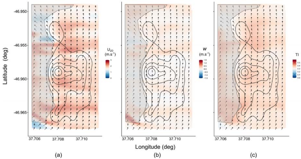
Fig. S9. Two-dimensional wind map, extracted at a constant 1 m.a.g.l. from numerical simulation of a southerly wind ( \theta = 180^\circ ) freestream condition over Marion Island. Crash site density contours (black, solid lines) are displayed with the outline of the base of the Ridge (semi-transparent grey area). Each grid point is denoted by an arrow indicating the wind direction (local wind direction) with backgrounds coloured by two-dimensional horizontal velocity magnitude ( U_{2D} ; a), the vertical wind component ( w ; b) and the isotropic turbulence intensity (TI; c)
